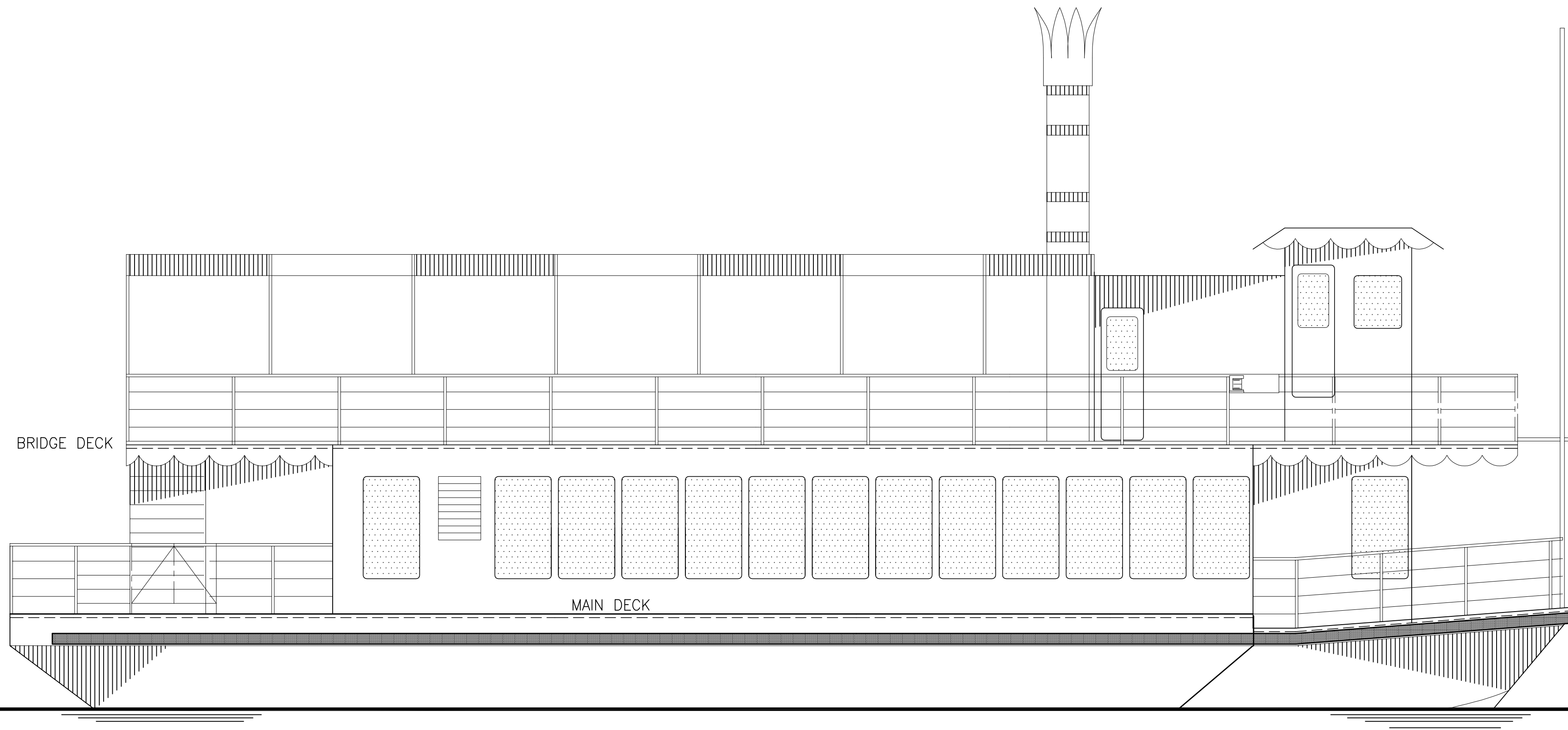
SHOWBOAT ROYAL GRACE ~ OUTBOARD PROFILE
